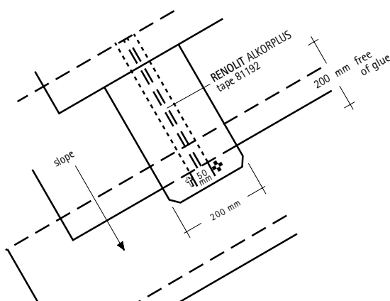
Fig. 1. transverse seams of roofing membrane
